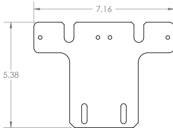
FLAT PATTERN
