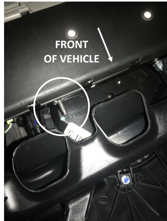
18) Locate the left most OEM bolt up behind the back of the glove box. Seen above with out a hex flange nut. (The hex flange nut will be installed on the OEM bolt before installation of 906-0989A Grand Caravan.)
