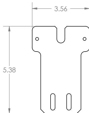
FLAT PATTERN
