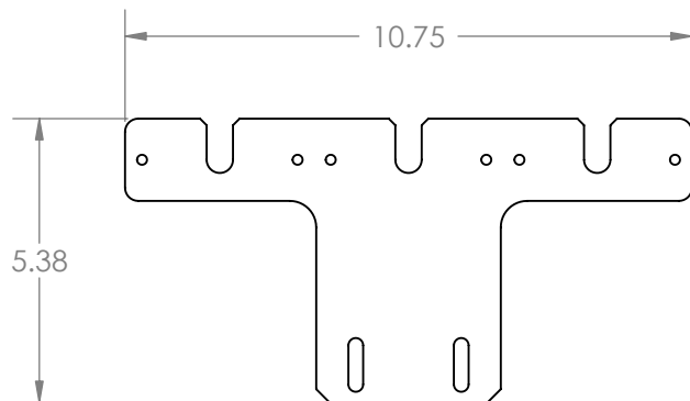
FLAT PATTERN
