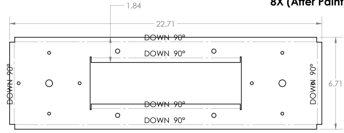
FLAT PATTERN
