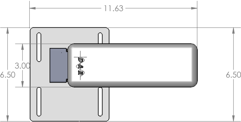
804-0545A Armrest Top Welding
