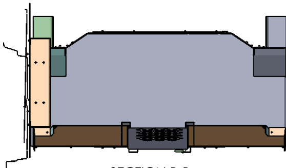
SECTION B-B SCALE 1 : 25
