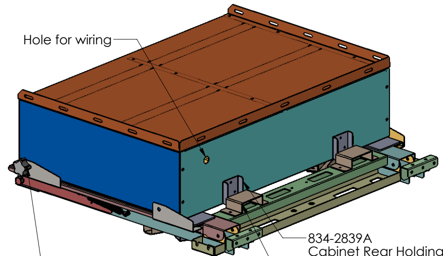
Both Side 3/8-16 Handle Bolt Cabinet with Subframe
