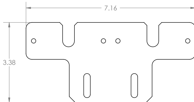
FLAT PATTERN
