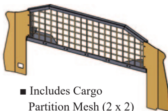
2021-2023 Ford Interceptor Utility Raised Subframe Partition (938-0150A)
